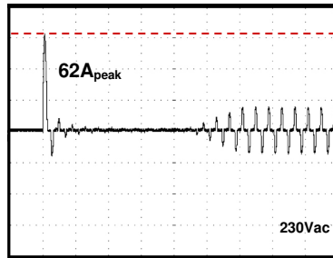
(Fig.5 inrush without ESB001)
